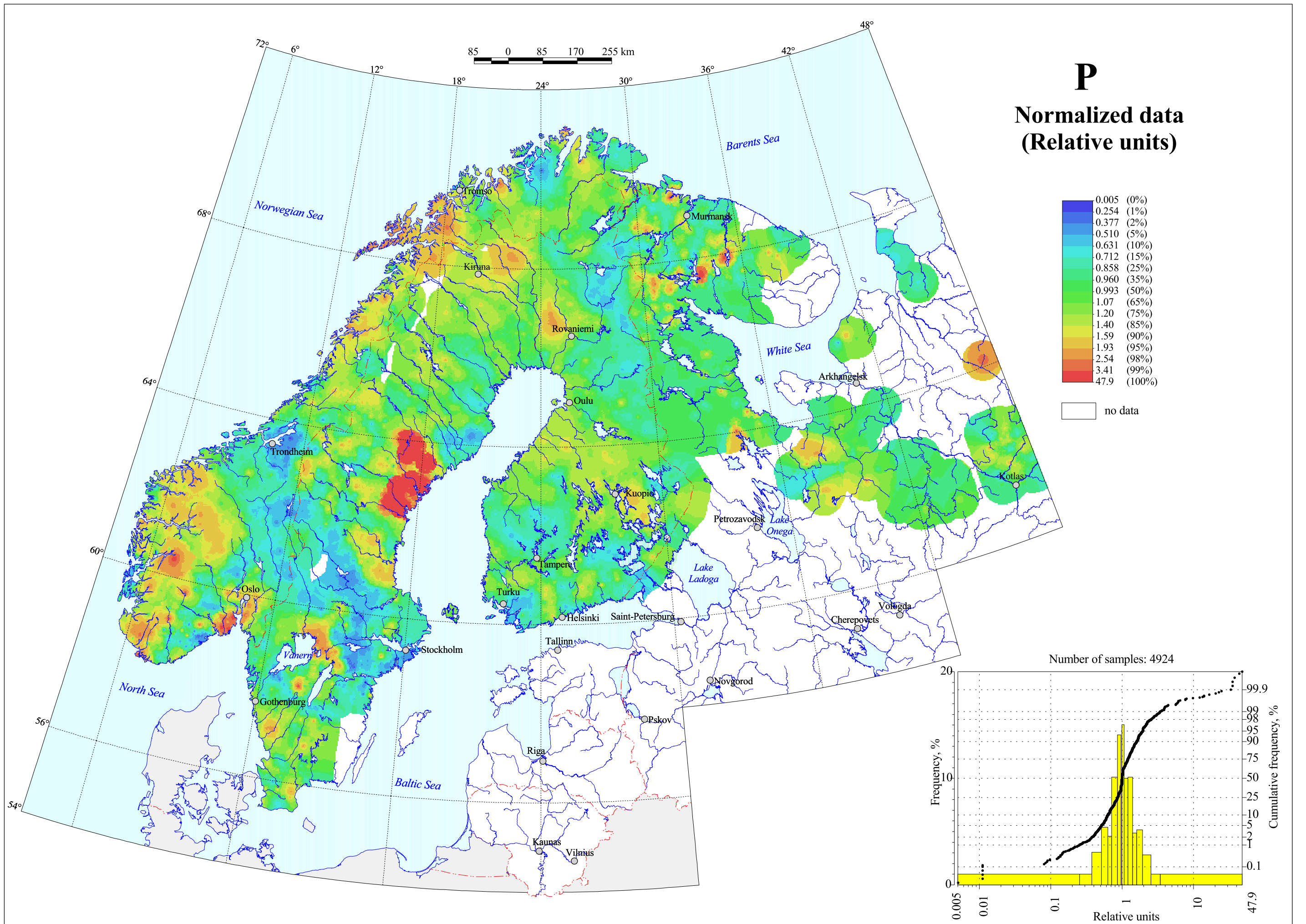
Phosphorus in Till, Grain Size <0.06 mm
